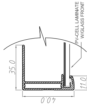
ALUMINUM FRAME B-B
