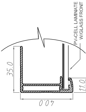
ALUMINUM FRAME B-B
