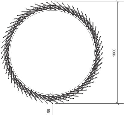
Plan View with direct attach
