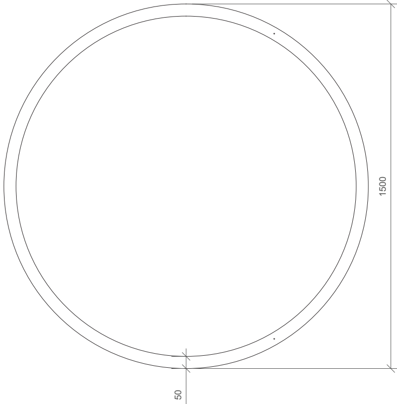
Plan View
