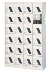
ASC-24WM (中棚付) ¥254,900(税抜) W1050×D380×H1700 ●内寸法:W226×D340×H248
