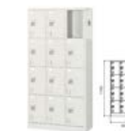
SG-12NK ¥173,700 (税別) W900×D380×H1790 ●内寸法(1マス): W248×D347×H397
