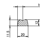
E-E'断面 E-E' cross section
