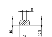
H-H'断面 H-H' cross section
