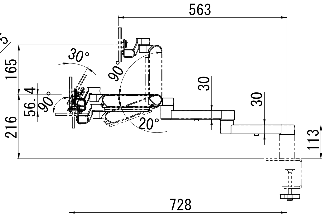
PS-N7B2+PS7-N900W
