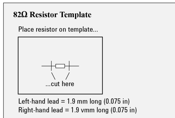
Figure 53 Resistor Trim Dimensions and Trim Gauge
