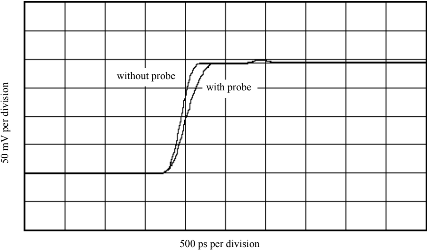
Figure 22 TDT measurement at receiver with and without probe load for 250 ps rise time
