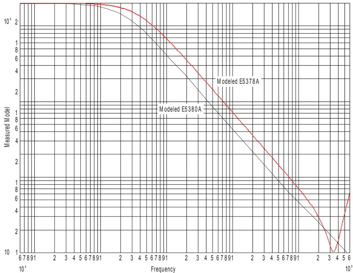
Measured versus modeled input impedance
