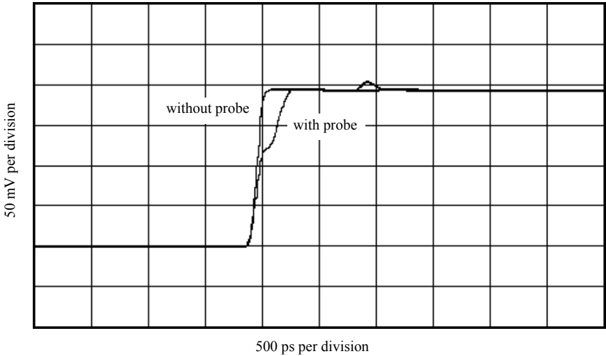
Figure 21 TDT measurement at receiver with and without probe load for 100 ps rise time
